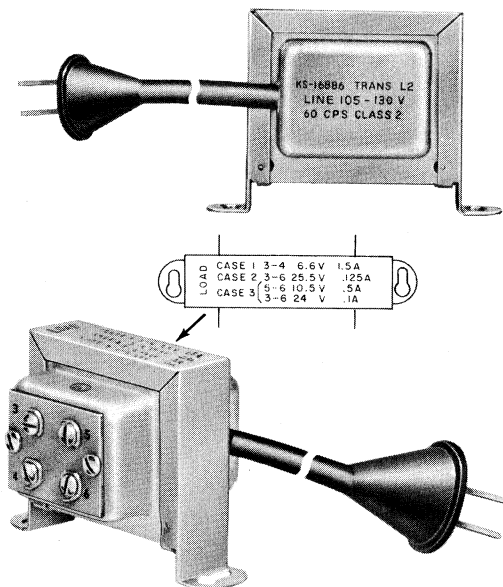
Fig. 8—KS-16886L2 Transformer
